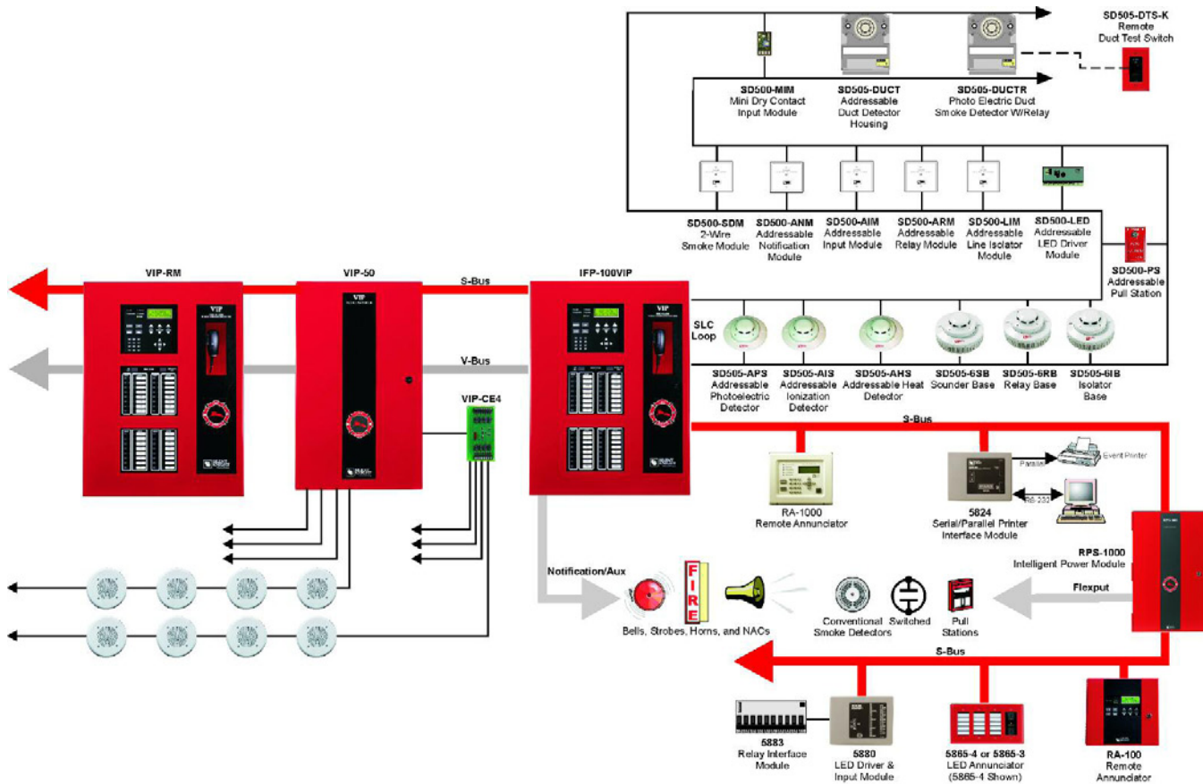
IFP-100VIP System Using Hochiki Protocol Devices on the SLC Loop
