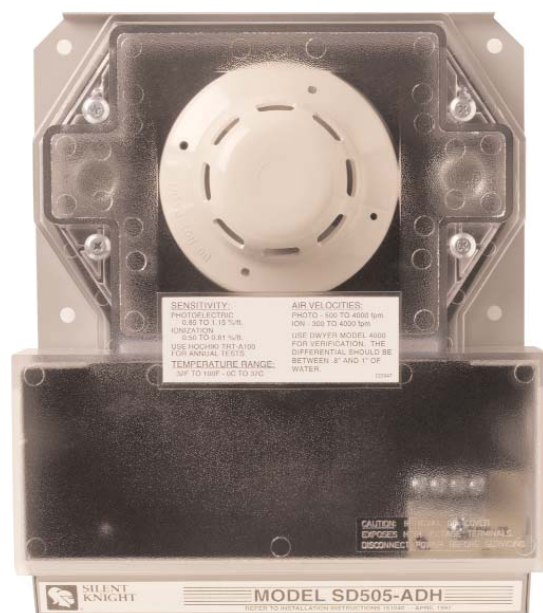
SD505-ADH Shown with Detector (Detector Sold Separately)
