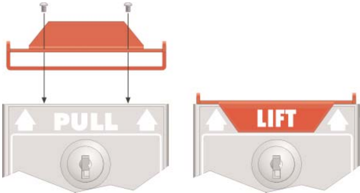
SD500-LK Installation
